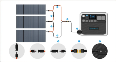
Panel MC4 to cable to station XT60
